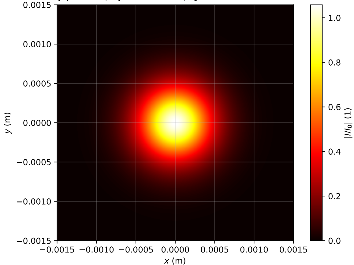
Intensity profile I(x, y, z = 0.876m)/I_0 , Pin=0.5Pcr, artificial time
